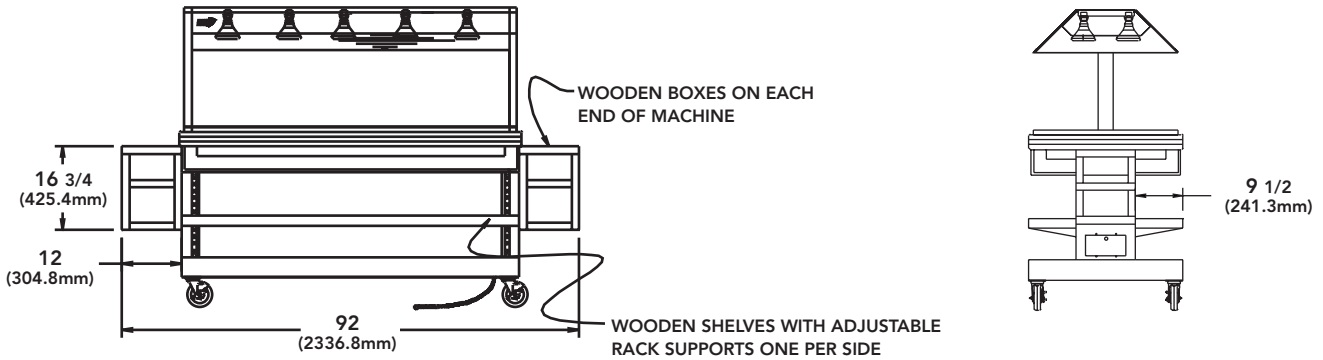
SHOWN WITH OPTIONAL RACKS AND SHELVES
